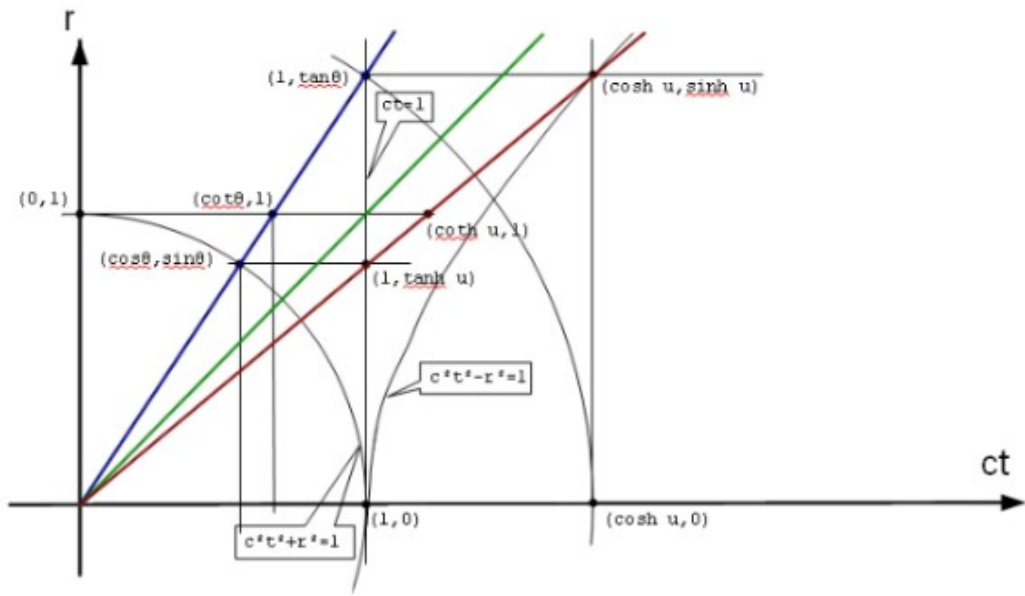
Hyperbolic Coordinate Construction
